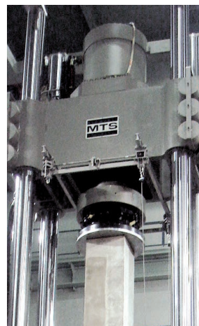
Compression Platens
